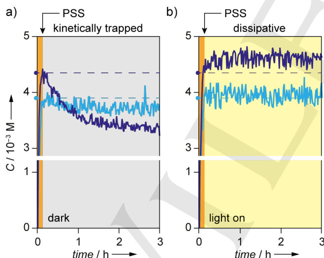
Figure 5. Time-dependent concentration profiles, determined by 1 H NMR, of complexed Z - 2a (cyan) and complexed Z - 2b (blue) quickly generated by 369 nm irradiation of an equilibrated mixture of the corresponding E axles and ring 1 . (a) Evolution of the kinetically trapped state in the dark. (b) Generation of a dissipative non-equilibrium state upon continuous irradiation. The orange bars mark the irradiation at high intensity to reach the PSS; the dashed lines indicate the corresponding concentration of the kinetically trapped Z complexes. Conditions: CD 3 CN, 298 K, [ 1 ] = [ 2a-b ] = 10 mM.
