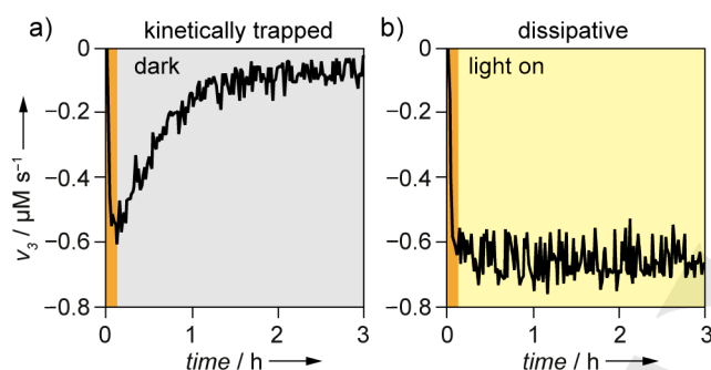
Figure 6. Threading rate of 1 and Z-2b as a function of time, calculated with equation 1 from experimentally determined rate constants (Table 2) and concentrations (Figure 5), in the dark (a) and under continued irradiation at 369 nm (b). In both cases, an equilibrated mixture of 1 and E-2b was rapidly brought to the photostationary state upon 369-nm irradiation. Conditions: CD 3 CN, 298 K, [ 1 ] = [ 2b ] = 10 mM.
