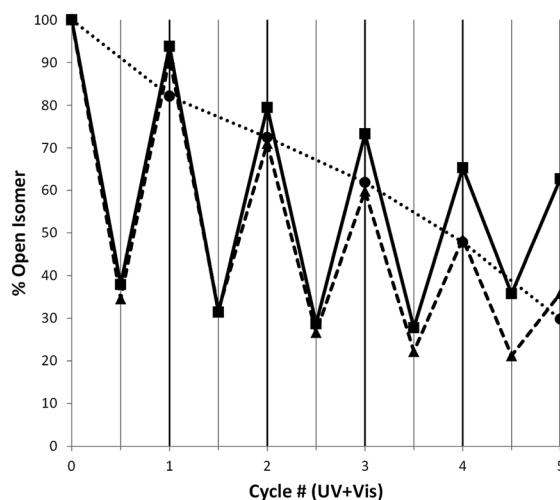
Fig. 5 Fatigue resistance of free axle [1_o\text{-H}]\text{BF}_4 (●, dotted line) [2]pseudorotaxane [1_o\text{-H}(\text{CE})]\text{BF}_4 (▲, dashed line; ■, solid line: 24C8 ) evaluated by ^1\text{H} NMR experiments (254 nm, \text{CD}_2\text{Cl}_2 , 0.02 M, 500 MHz, 298 K).
