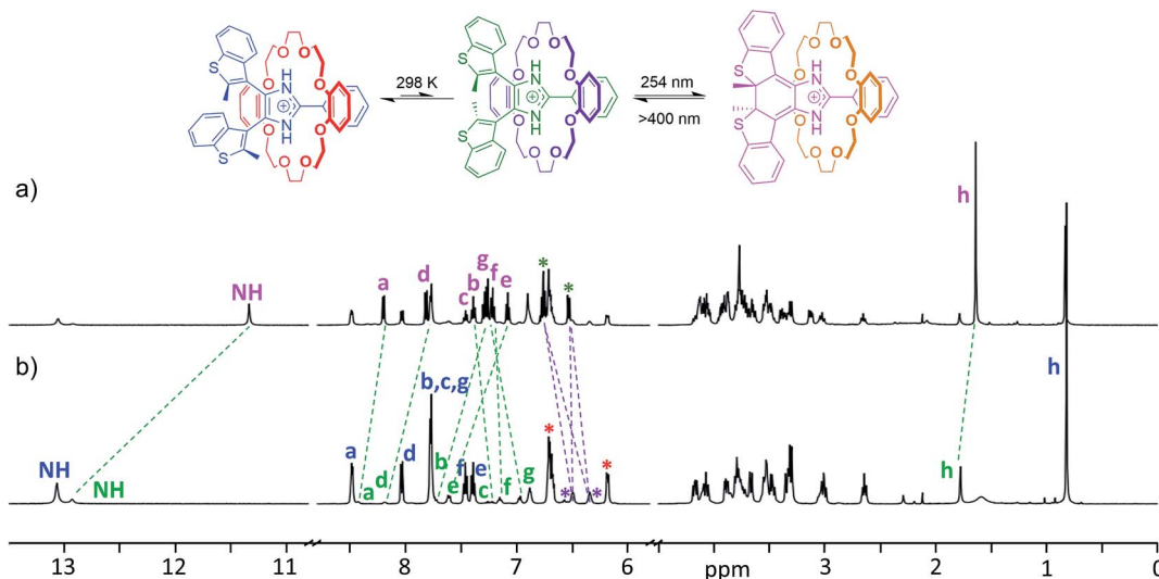
Fig. 6 ^1\text{H} NMR spectra of (a) [1_{\text{c}}-\text{H}<\text{DB24C8}]\text{BF}_4 after reaching the photostationary state by irradiation with 254 nm light for 10 min, and (b) [1_{\text{o}}-\text{H}<\text{DB24C8}]\text{BF}_4 [2]pseudorotaxane ( \text{CD}_2\text{Cl}_2 , 500 MHz, 298 K). Corresponding peaks are matched by dashed lines; the axle peaks and the aromatic peaks of the macrocycle are labelled using colours matching the accompanying reaction scheme.
