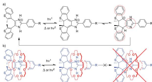
Scheme 3 Proposed photoisomerization and cycloreversion pathways for (a) free axles [1-3-\text{H}]^+ , and (b) [2]pseudorotaxanes [1-3-\text{H}<(\text{CE})]^+ .
